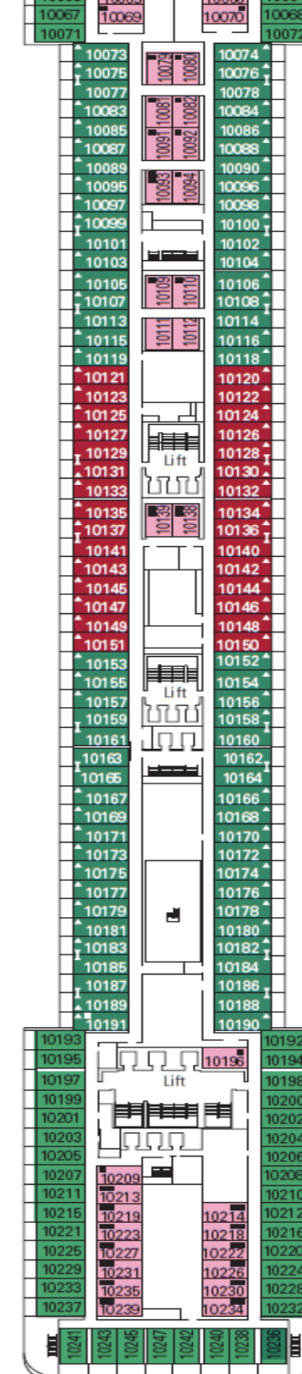
DECK 10 CARDUCCI
